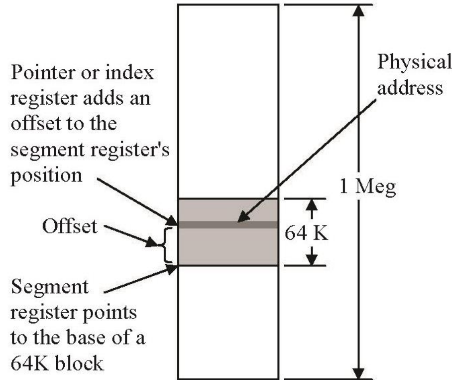
Figure 16-3 Segment/Pointer Relation in the 80x86 Memory Map
