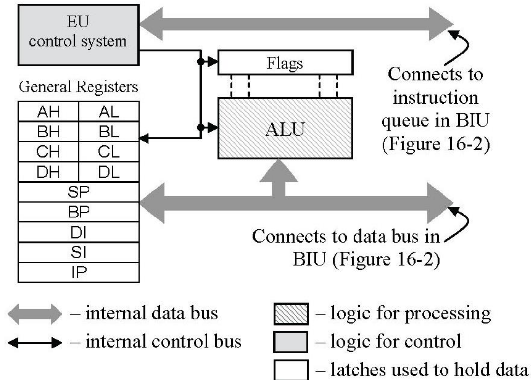
Figure 16-1 Block Diagram of 80x86 Execution Unit (EU)
